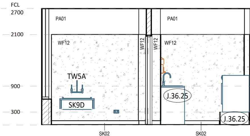
3 ELEVATION DETAIL 1 : 50
