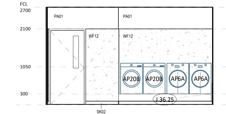
4 ELEVATION DETAIL 1 : 50
