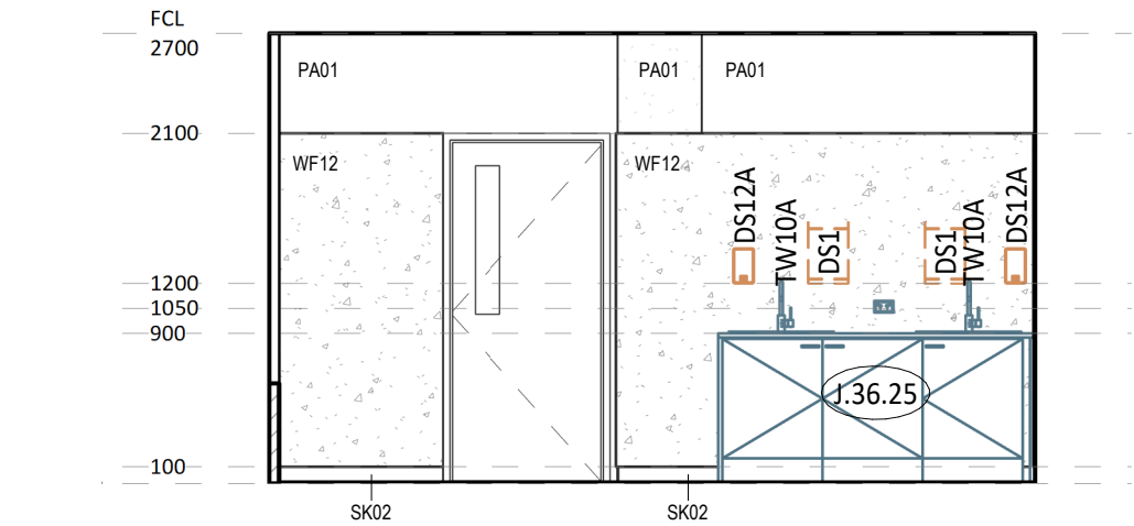
2 ELEVATION DETAIL 1 : 50
